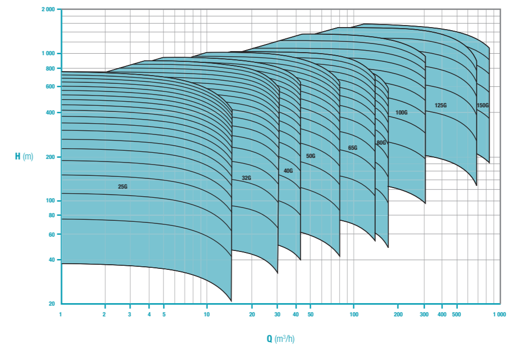
PERFORMANCE CURVE - 60HZ / 3500 RPM
