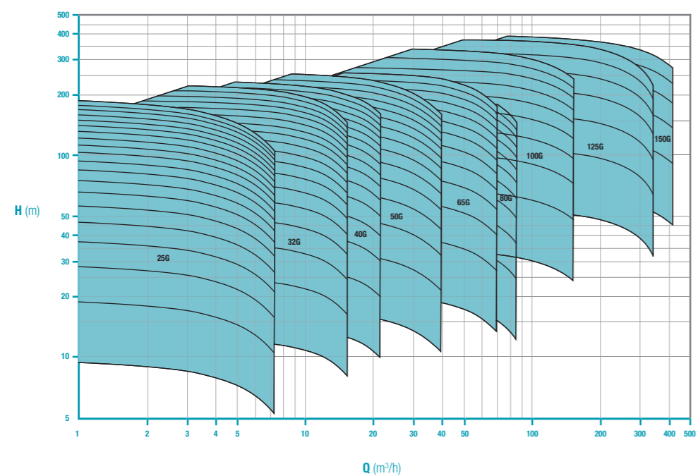
PERFORMANCE CURVE - 60HZ / 1750 RPM
